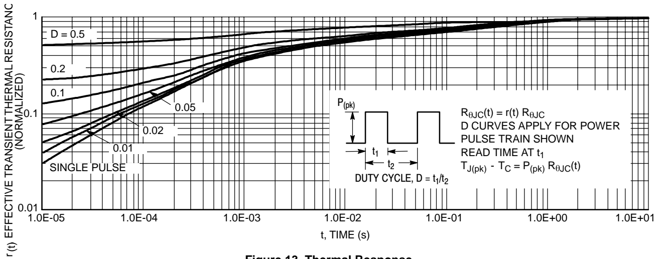
Figure 13. Thermal Response
